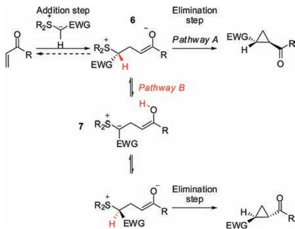
Scheme 5. Proposed Pathways Leading to Cyclopropanes from Enones
