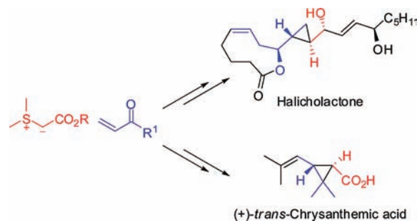
Scheme 4. Asymmetric Cyclopropanations of Acyclic Enones with Ester-Stabilized Ylide 1b
